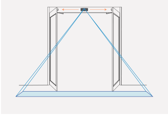
Mounting on swing doors - flexible mounting position.
